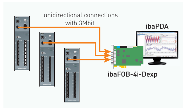
Connecting several ibaPADU devices via unidirectional F0 connections with 3Mbit protocol
