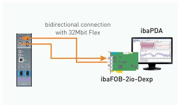
Connecting a bus monitor via a bidirectional F0 connection with 32Mbit Flex protocol
